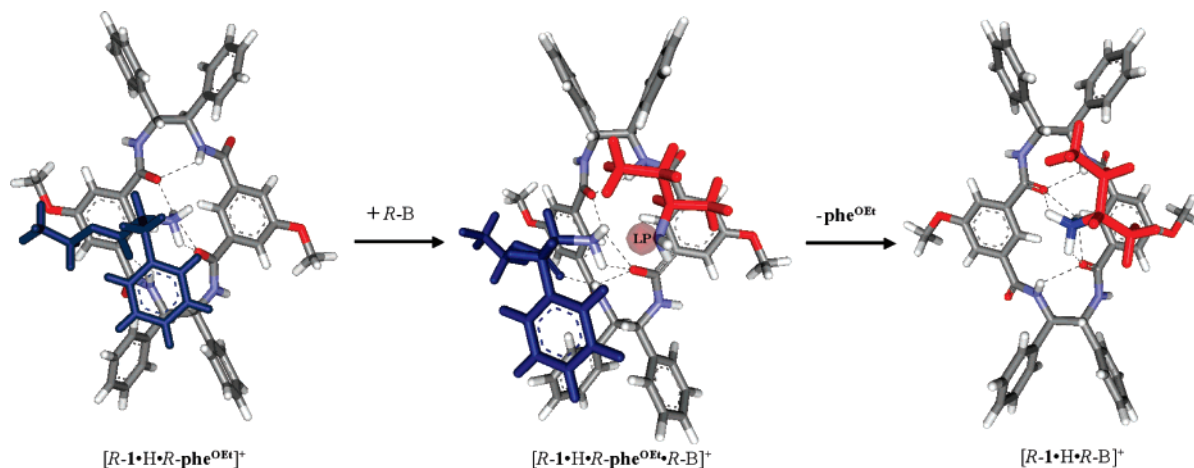
Figure 5. Simulation by docking experiments of the r\text{-phe}^{\text{OEt}} displacement from the [r\text{-1}\cdot\text{H}\cdot r\text{-phe}^{\text{OEt}}]^+ complex by \text{Br} . The most stable structure of the protonated trimer [r\text{-1}\cdot\text{H}\cdot r\text{-phe}^{\text{OEt}}\cdot\text{Br}]^+ , obtained by docking procedure, is depicted in the center (LP is the lone-pair of \text{Br} ).
